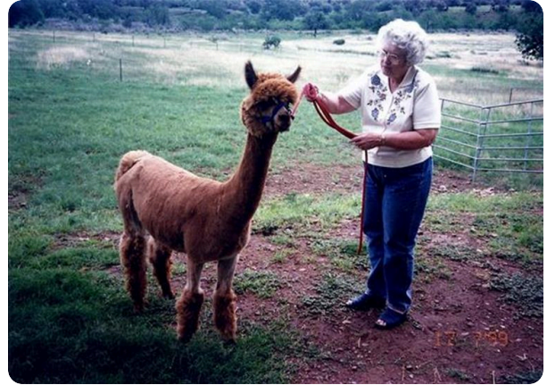
Alpaca Farm
